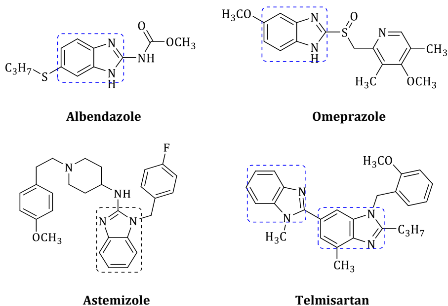
Figure 1. Some currently used drugs containing benzimidazole nucleus
