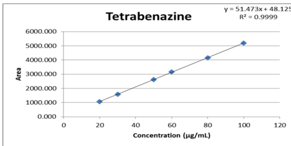
Figure 4. Calibration curve for Tetrabenzazine.
