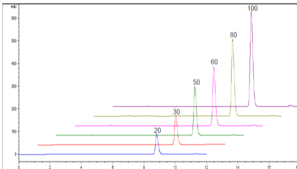
Figure 3. Chromatograms of Tetrabenzazine in various concentrations for linearity test.
