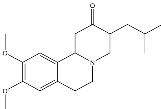
Figure 1. Chemical structure of Tetrabenazine.
