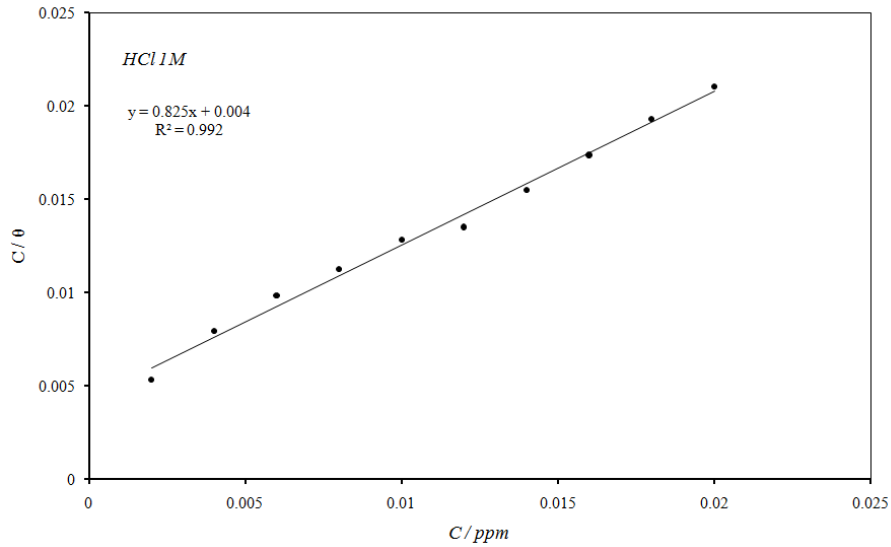
Figure 3. Langmuir adsorption plots for carbon steel in 1 M HCl containing various concentrations of the Salen at 25°C
