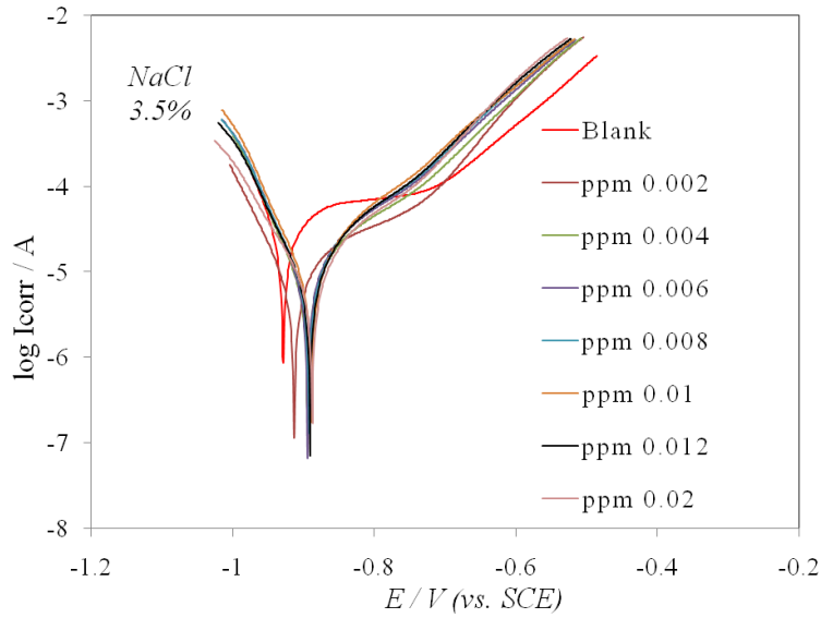
Figure 2. Potentiodynamic polarization curves for Salen in NaCl 3.5% with and without different concentrations of Salen at 20°C (immersion time is 2 h)
