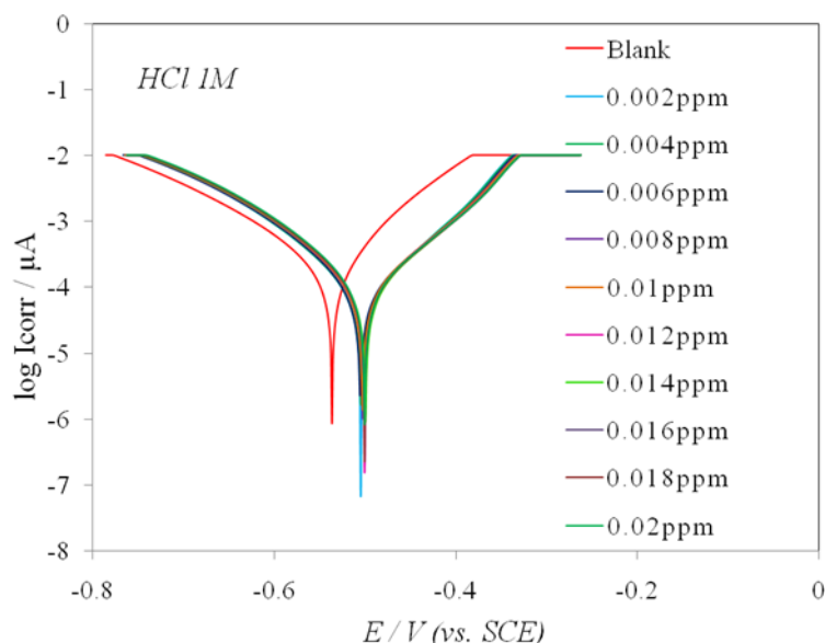
Figure 1. Potentiodynamic polarization curves for Salen in 1.0 M HCl with and without different concentrations of Salen at 20°C (immersion time is 2 h)
