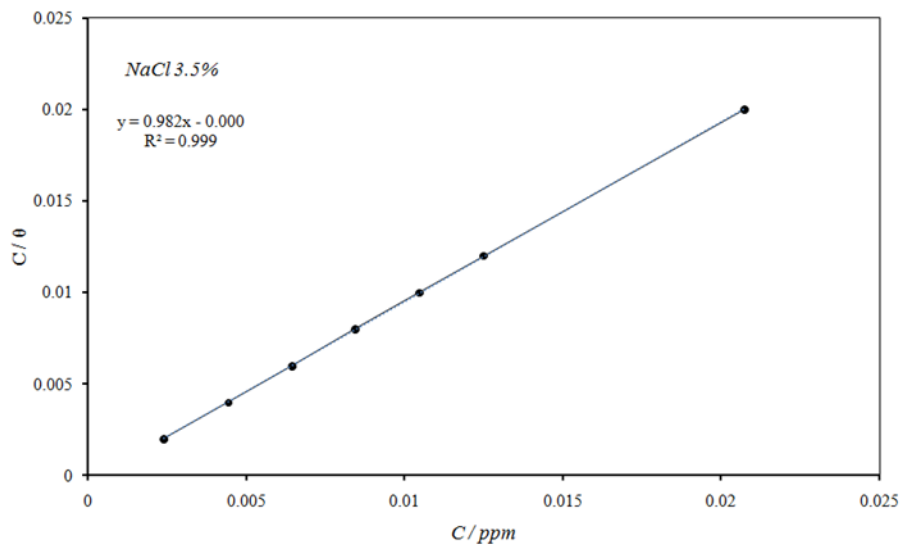
Figure 4. Langmuir adsorption plots for carbon steel in 3.5% NaCl containing various concentrations of the Salen at 25°C
