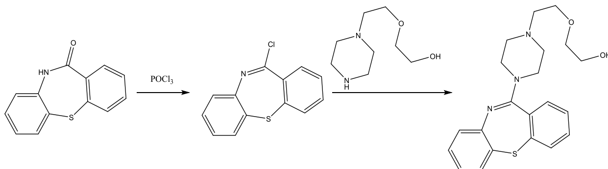
Figure 2. Quetiapine synthesis of dibenzo[b,f][1,4]thiazepine-11(10-H)-one and POCl 3
