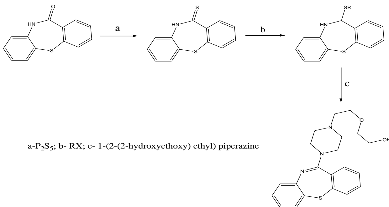
Figure 3. Quetiapine synthesis of dibenzo[b,f][1,4]thiazepine-11(10-H)-one and P 2 S 5
