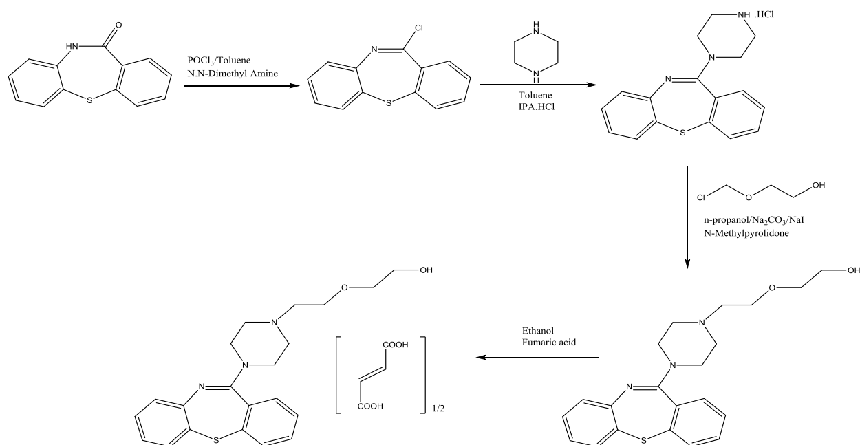
Figure 4. Quetiapine hemifumarate synthesis
