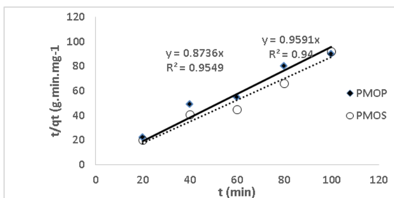
Figure 2: Pseudo-second-order kinetics for chromium adsorption on PMOS and PMOP adsorbents
