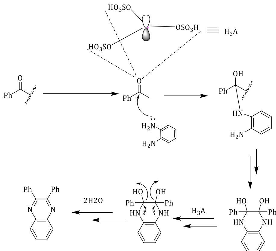
Scheme 2. Suggested mechanism for quinoxaline synthesis
