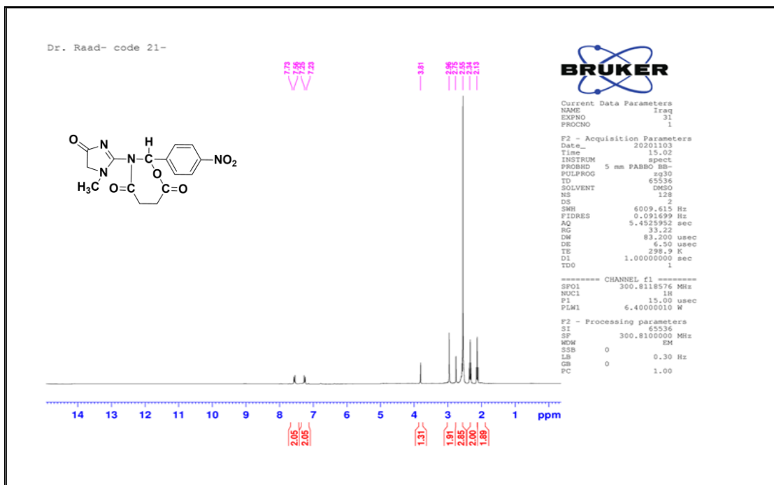
Figure 9: 1 H-NMR spectrum for compound [4a]
