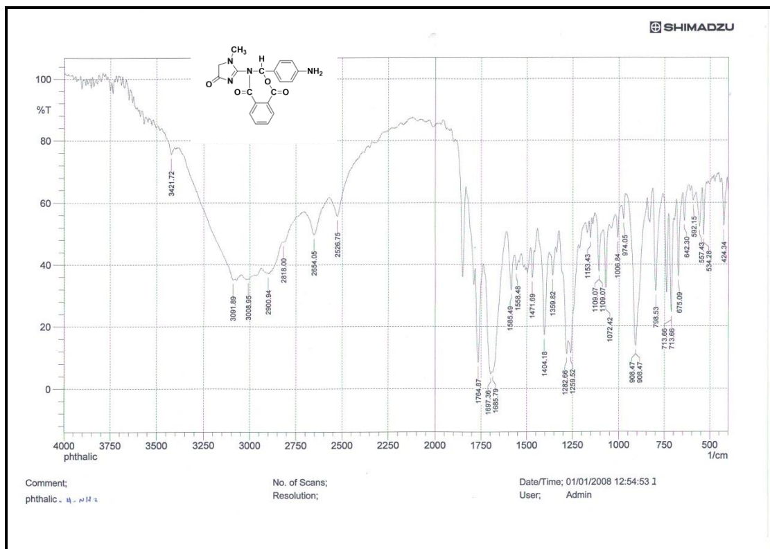
Figure 4: FT-IR spectrum for compound [2b]
