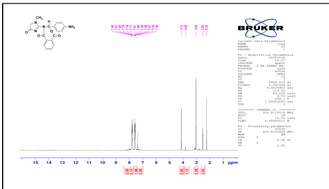
Figure 5: 1 H-NMR spectrum for compound [2b]
