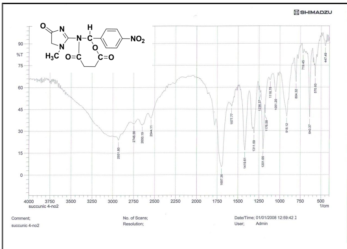
Figure 8: FT-IR spectrum for compound [4a]
