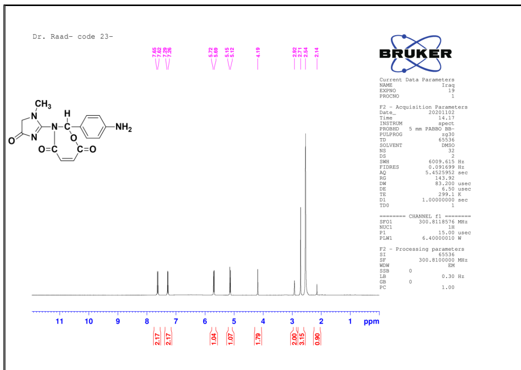
Figure 7: ^1\text{H-NMR} spectrum for compound [3b]
