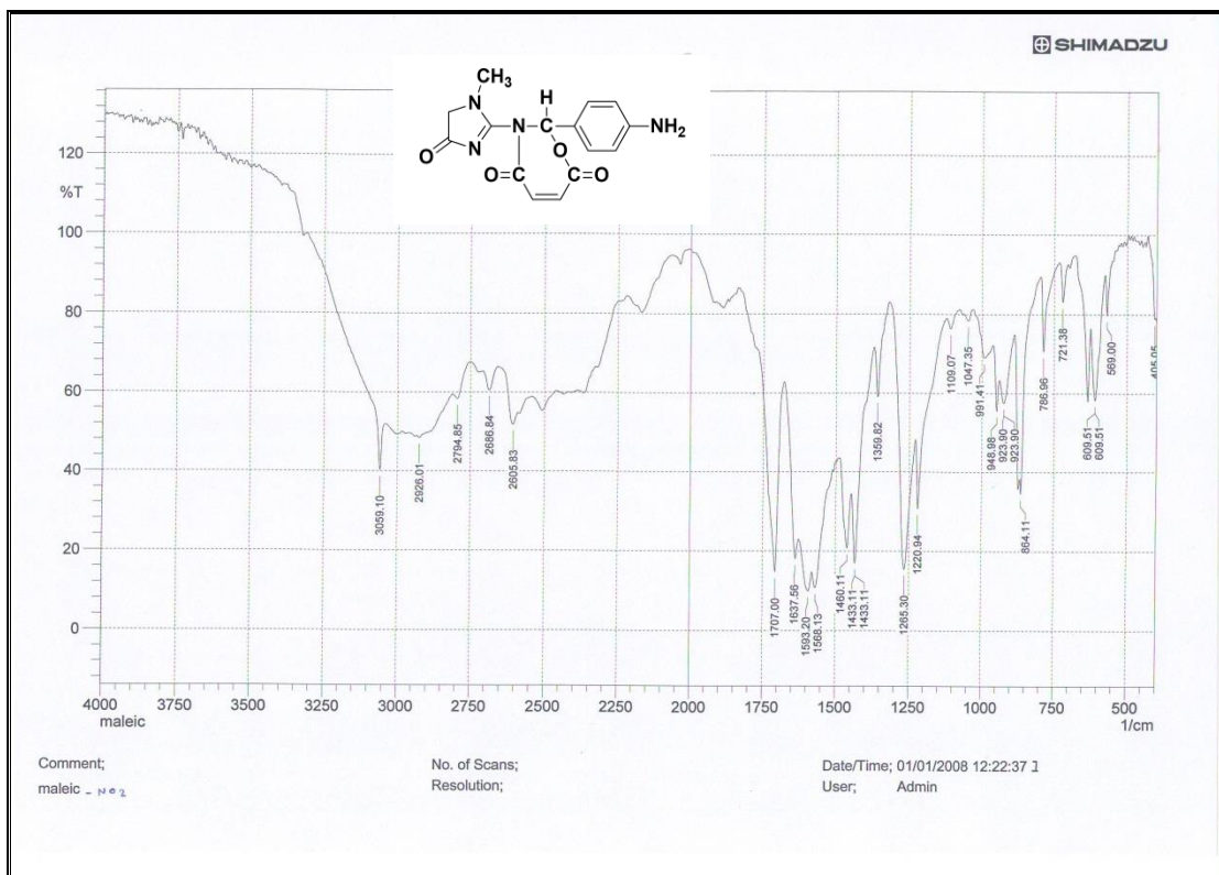
Figure 6: FT-IR spectrum for compound [3b]
