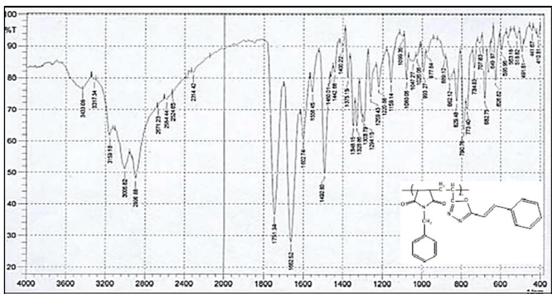
Figure 10: FT-IR spectrum for compound [17]
