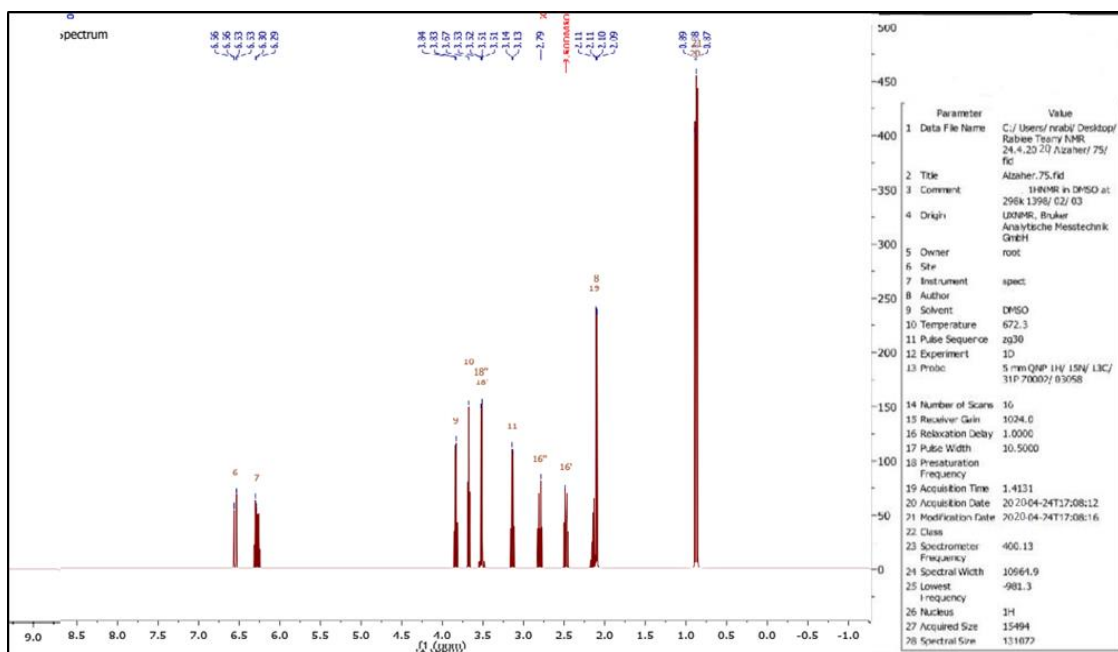
Figure 5: ^1\text{H} NMR spectrum for compound [19]
