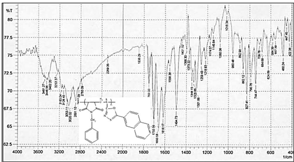
Figure 9: FT-IR spectrum for compound [16]
