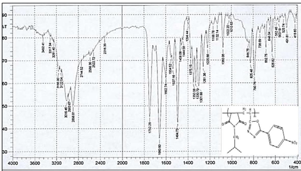
Figure 11: FT-IR spectrum for compound [24]
