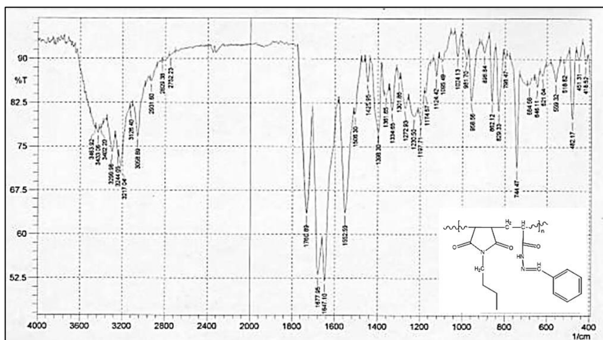
Figure 8: FT-IR spectrum for compound [11]
