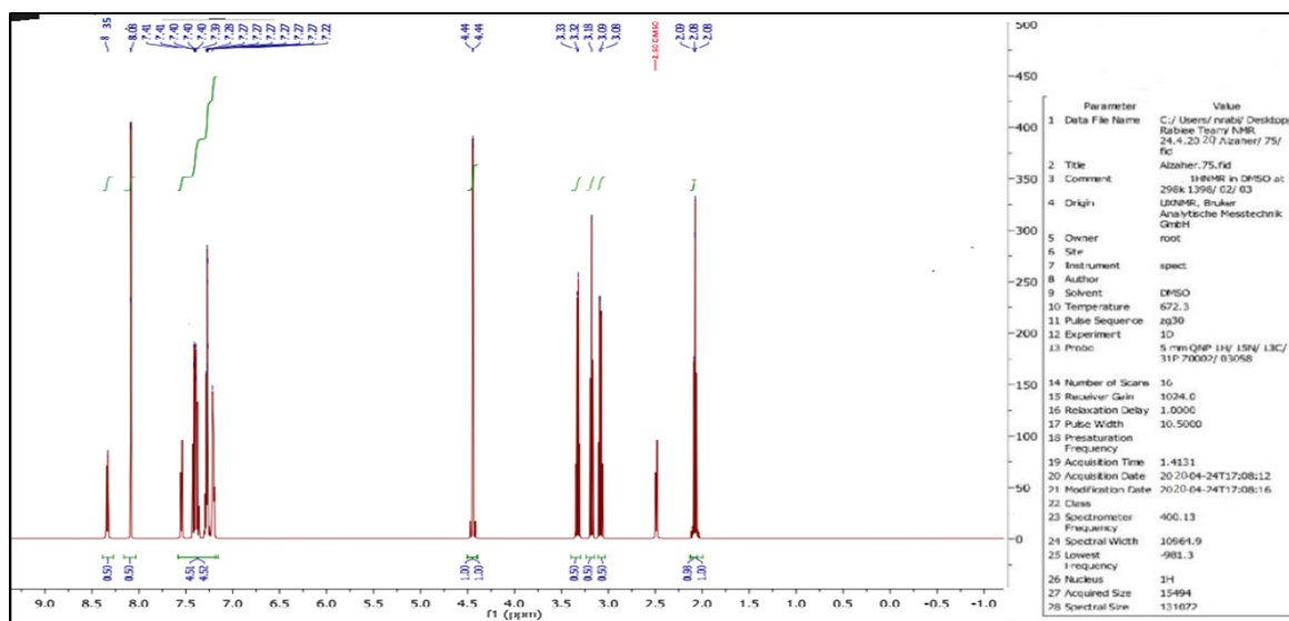
Figure 3: 1 H NMR spectrum for compound [2]
