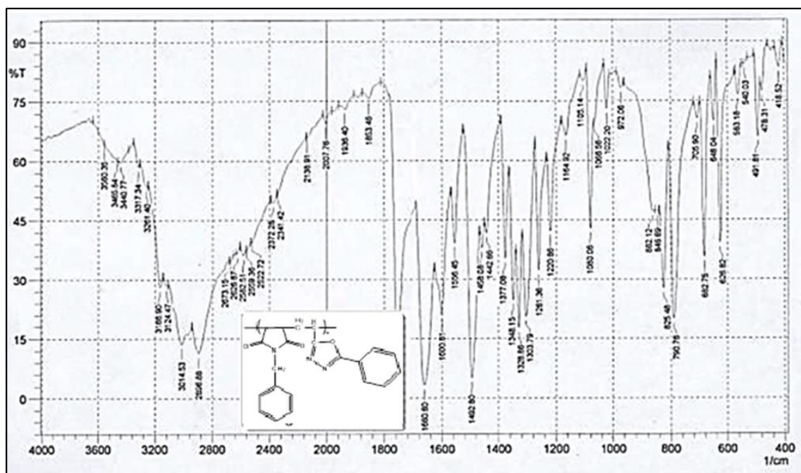
Figure 12: FT-IR spectrum for compound [29]
