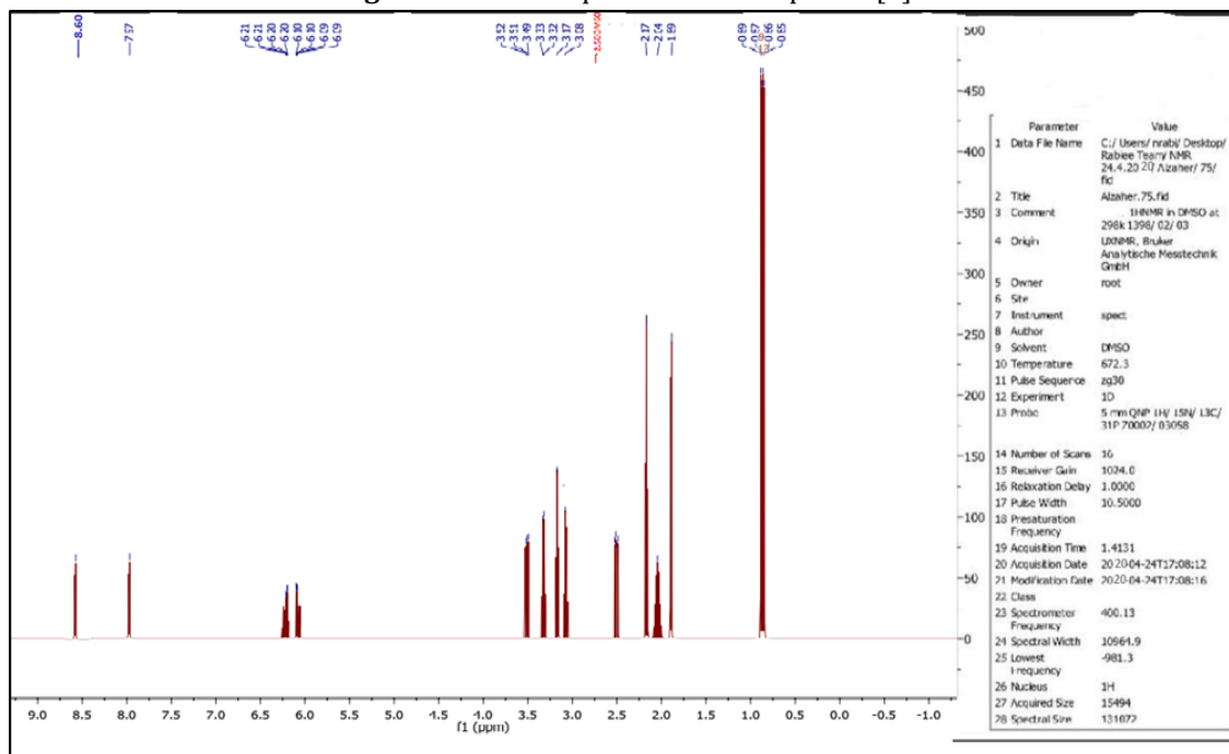
Figure 4: 1 H NMR spectrum for compound [5]
