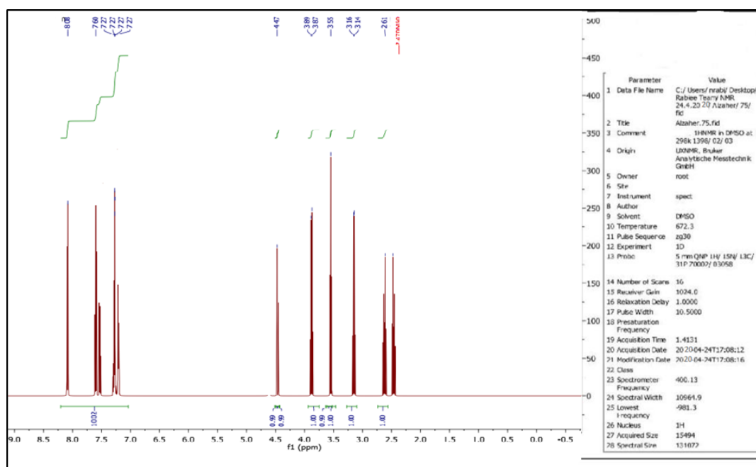
Figure 6: ^1\text{H} NMR spectrum for compound [29]
