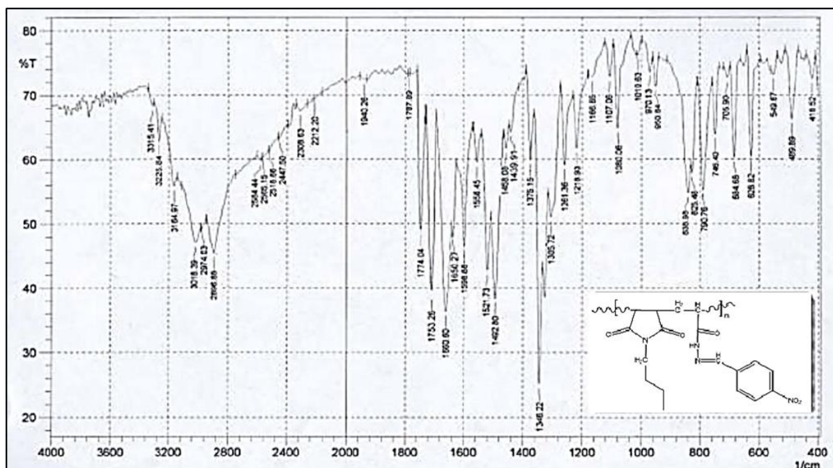
Figure 7: FT-IR spectrum for compound [8]
