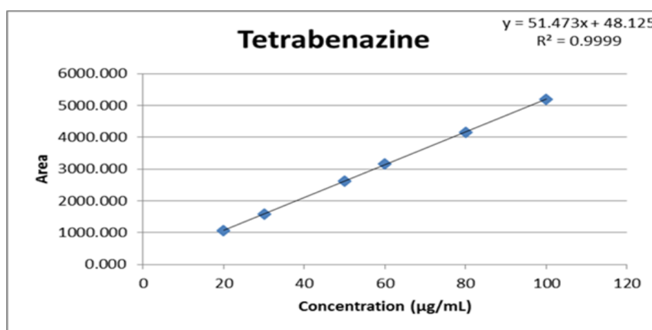
Figure 4. Calibration curve for tetrabenazine
