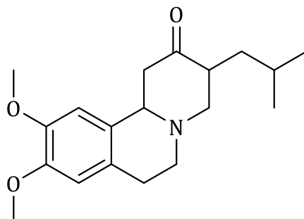
Figure 1. chemical structure of tetrabenazine
