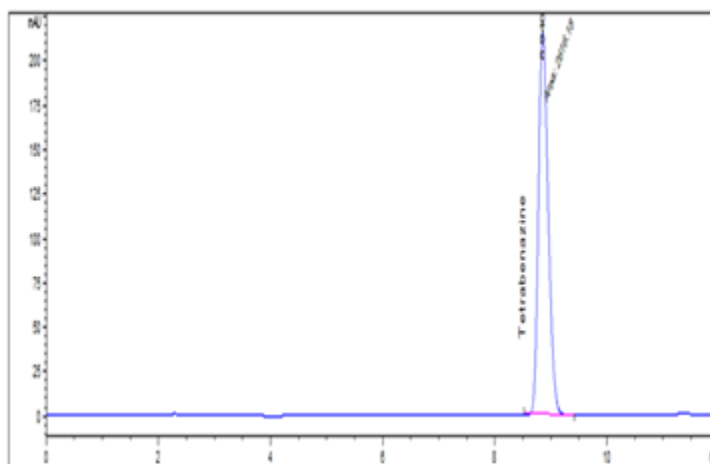
Figure 2. chromatogram of tetrabenazine
