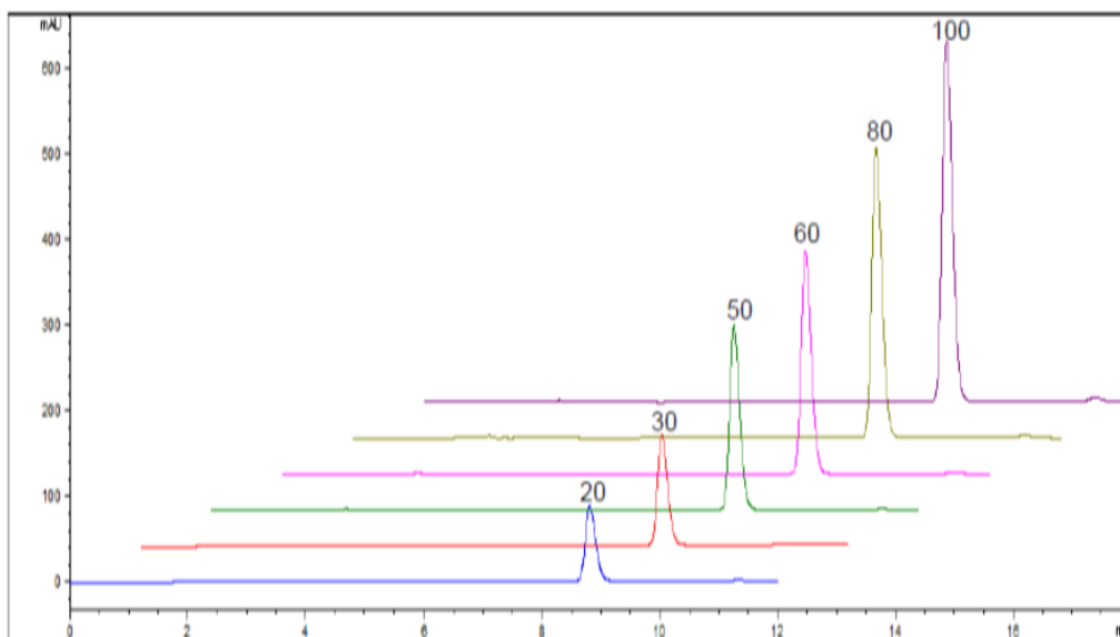
Figure 3. Chromatograms of tetrabenazine in various concentrations for linearity test
