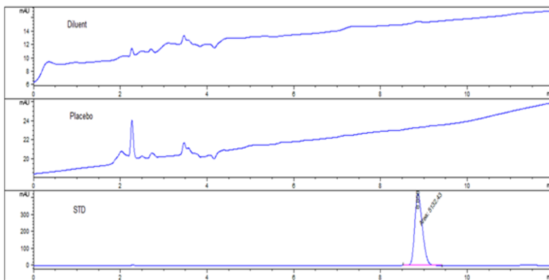
Figure 5. Diluent, placebo and standard solution chromatogram
