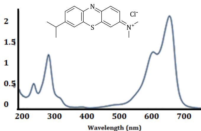
Scheme 1: Structure and UV-vis spectrum of methylene blue
