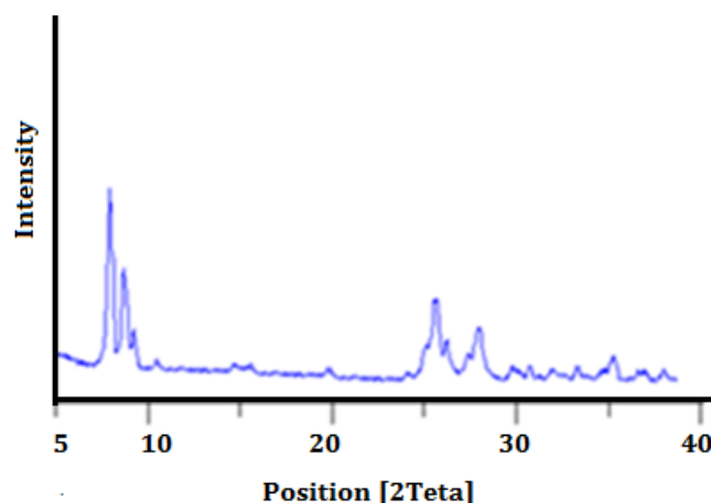
Figure 5: XRD patterns of TBA-PMoV
