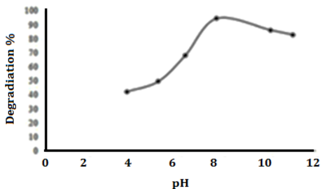
Figure 7: Effect of pH on photocatalytic degradation of methylene blue
