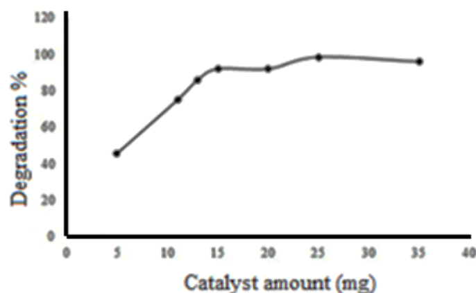
Figure 8: Effect of catalyst amount on photocatalytic degradation of methylene blue
