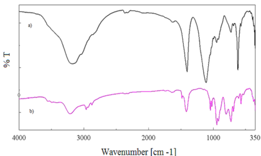
Figure 1: FT-IR spectrum of a) fresh PMoV and b) TBA-PMoV
