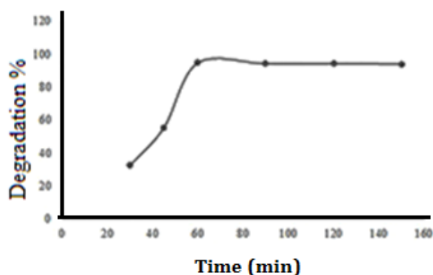
Figure 6: Effect of time on photocatalytic degradation of methylene blue
