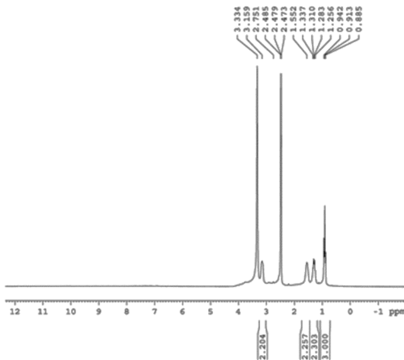
Figure 4: 1 HNMR spectrum of TBA-PMoV
