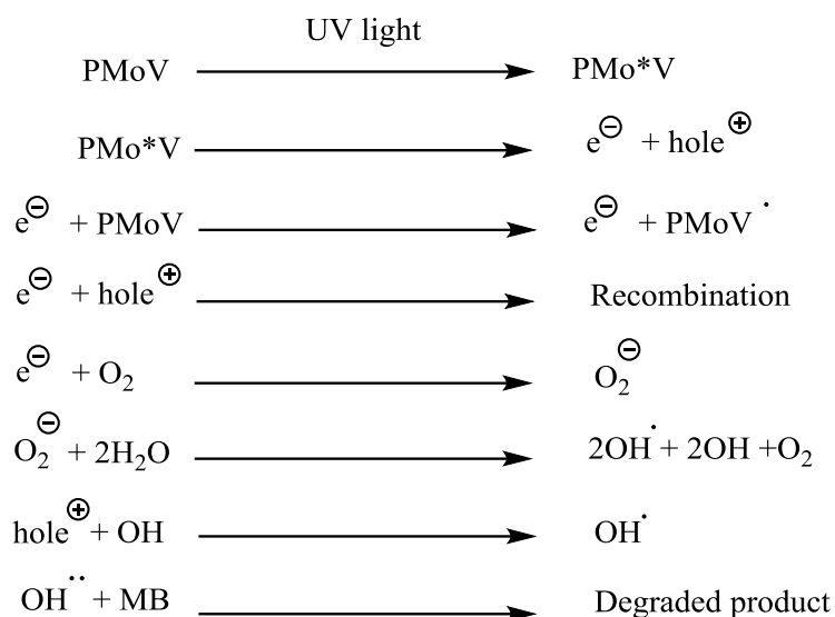
Scheme 2: Proposed mechanism for degradation of MB by catalyst
