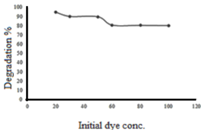
Figure 9: Effect of initial concentration of dye on the photocatalytic degradation of methylene blue, C_0=x mg/L, pH=7.6, Time=60 min
